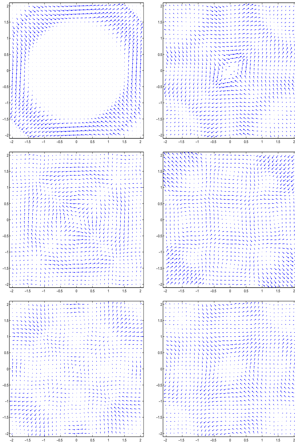
FIG. 6.8. Scaled first two components of \mathbf{U}(t, \cdot) for the solution provided by Algorithm 3.1 for equivariant initial data for t \approx 0, 2.0, 4.0, 6.0, 8.0, 10.0 .
