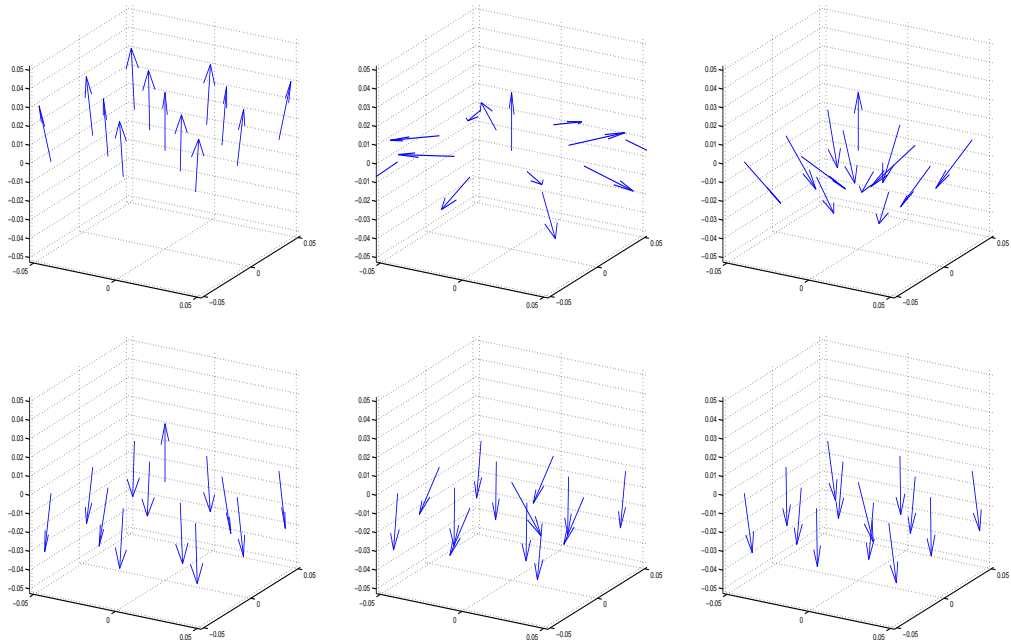
FIG. 6.4. Scaled solution \mathbf{U}(t, \cdot) obtained with Algorithm 3.1 in a neighborhood of the origin for t = 0, 0.20025, 0.40051, 0.60076, 0.80102, 1.00130 on a criss-cross triangulation.
