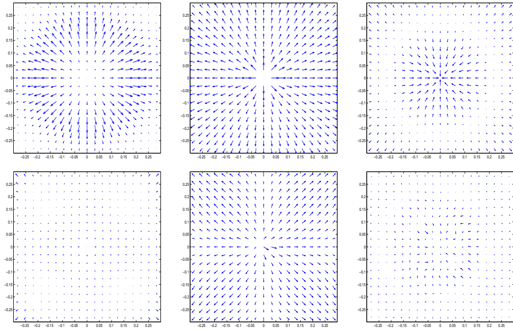
FIG. 6.3. Scaled first two components of \mathbf{U}(t, \cdot) for the solution provided by Algorithm 3.1 for t = 0, 0.20025, 0.40051, 0.60076, 0.80102, 1.00130 .
