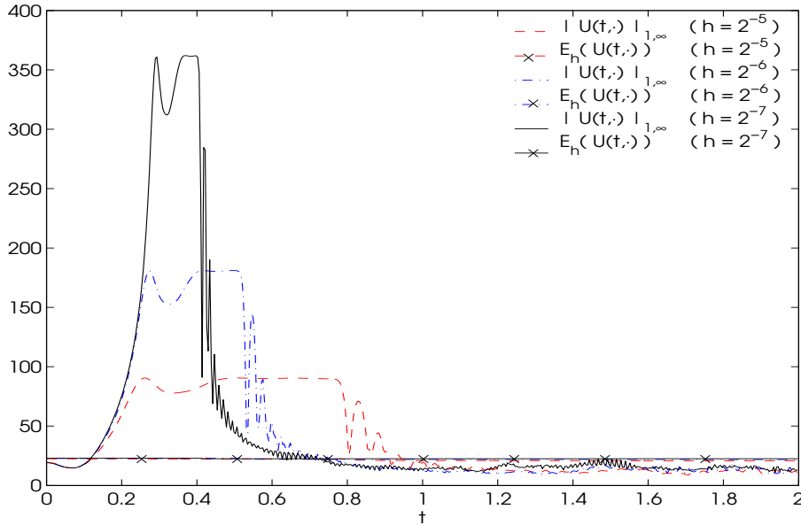
FIG. 6.2. W^{1,\infty} seminorm and discrete energy as functions of t \in [0, 2] for approximations obtained with Algorithms 3.1 on refining triangulations.
