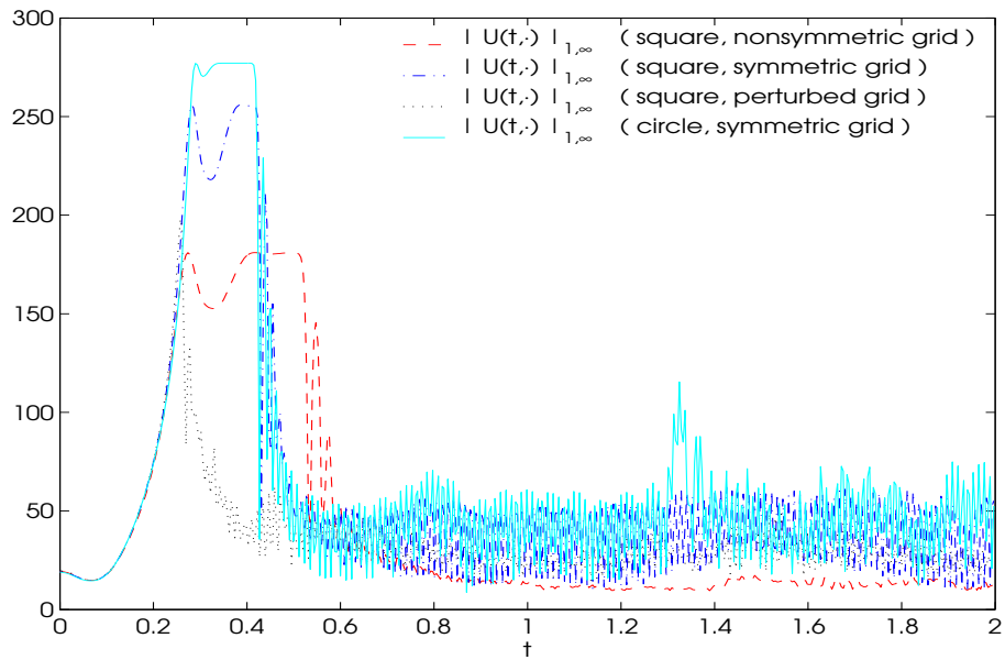
FIG. 6.6. W^{1,\infty} semi norm and discrete energy as functions of t \in [0, 2] for approximations obtained with Algorithm 3.1 for (refinements of) the triangulations shown in Figure 6.5.
