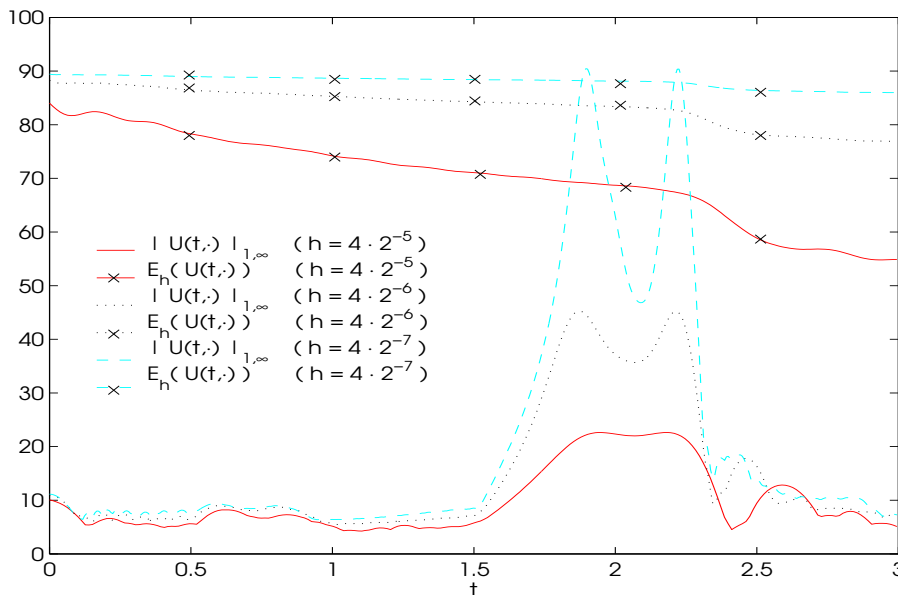
FIG. 6.7. W^{1,\infty} seminorm and discrete energy as functions of t \in [0, 3] for approximations obtained with Algorithms 3.1 for equivariant initial data on refining triangulations.
