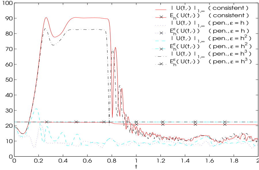
FIG. 6.1. W^{1,\infty} seminorm and discrete energy as functions of t \in [0, 2] for approximations obtained with Algorithms 3.1 and 3.2 for various choices of \epsilon .
