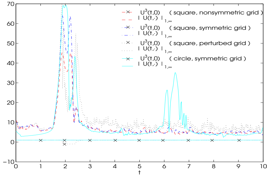
FIG. 6.9. W^{1,\infty} seminorm and third component of numerical solutions at origin of t \in [0, 10] for approximations obtained with Algorithm 3.1 for (refinements of) the triangulations shown in Figure 6.5 and equivariant initial data.
