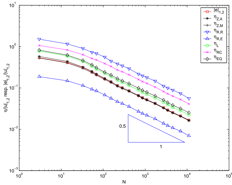
FIGURE 10. Relative error and error estimators for \eta_{R,R} adaptive mesh refinement in Example 8.3.
