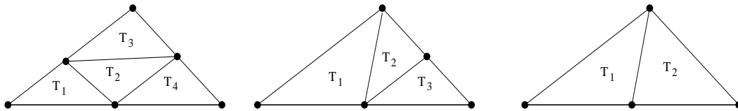
FIGURE 3. Red-, blue-, and green-refinement of a triangle.
