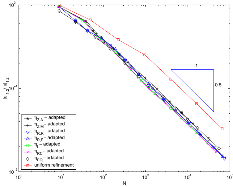
FIGURE 8. Relative error on a uniform and on adaptively refined meshes in Example 8.2.
