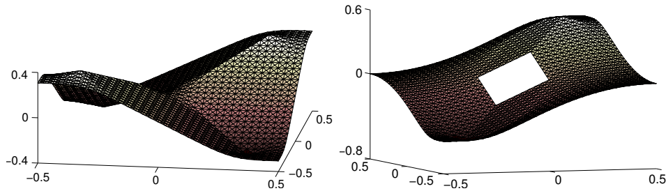
FIGURE 3. Approximate potentials \phi_h on the initial triangulations of convex (left) and nonconvex (right) domains in Examples 6.1 and 6.2.
