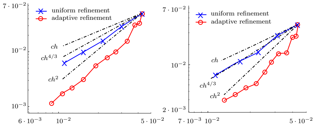
FIGURE 5. Primal-dual gap \delta_h with extrapolated reference value K_{ref} in the modified versions of Examples 6.1 and 6.2.
