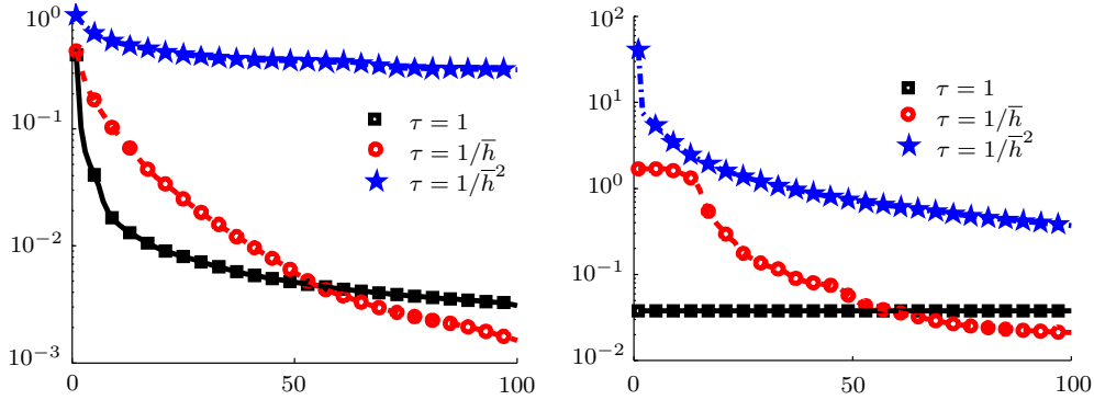
FIGURE 7. Convergence of the discrete residual for the primal (left) and dual (right) splitting algorithms on a fixed triangulation resulting from 12 uniform refinements and different step sizes.
