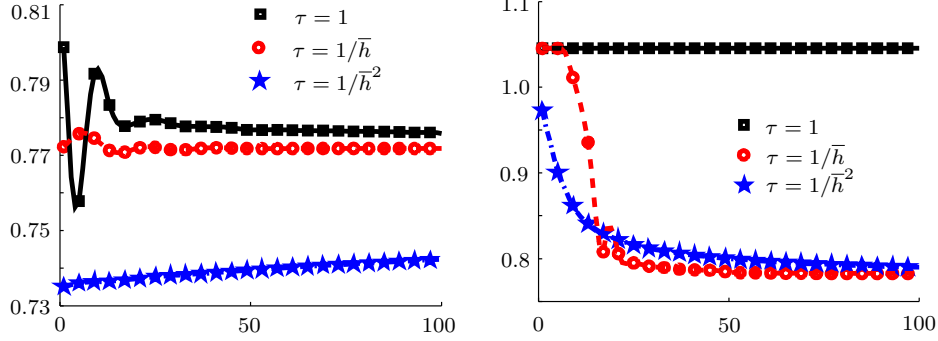
FIGURE 8. Convergence of the primal (left) and dual (right) cost functionals during the iteration of the primal and dual splitting algorithms.
