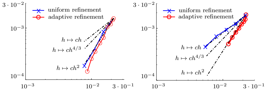
FIGURE 2. Approximated primal cost errors K_{ref} - K_h(\phi_h) in the convex (left) and nonconvex (right) settings from Examples 6.1 and 6.2. Adaptive mesh refinement leads to reduced errors and an improved experimental convergence rate in the nonconvex setting.
