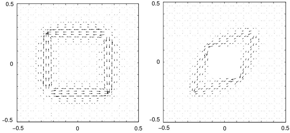
FIGURE 4. Approximated transport flux on a convex (left) and a nonconvex (right) domain. Nearly no transport occurs through the center of the convex domain.
