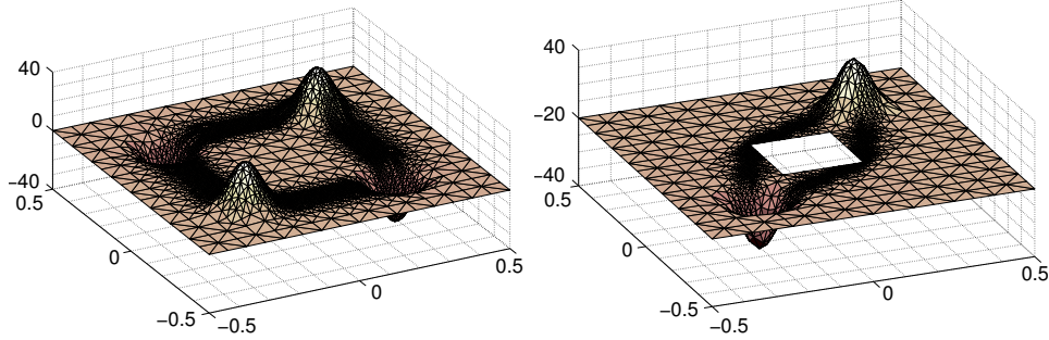
FIGURE 1. Density functions f = f^+ - f^- in Examples 6.1 (left) and 6.2 (right) on adaptively generated triangulations.
